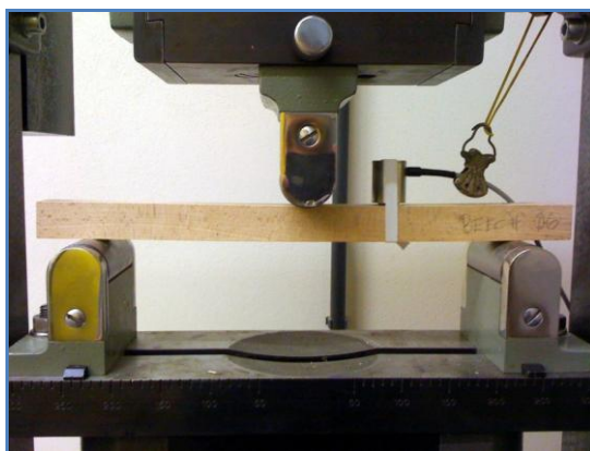
Figure 1: Position of a wood specimen on the bending test machine. Note the AE 767 acoustic emission sensor attached to the specimen via a rubber band and secured against fall-down using a security clamp.
