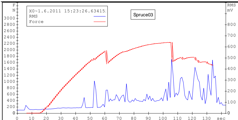
Figure 3: Typical plot of loading force vs. AE RMS for SPRUCE specimen group.
