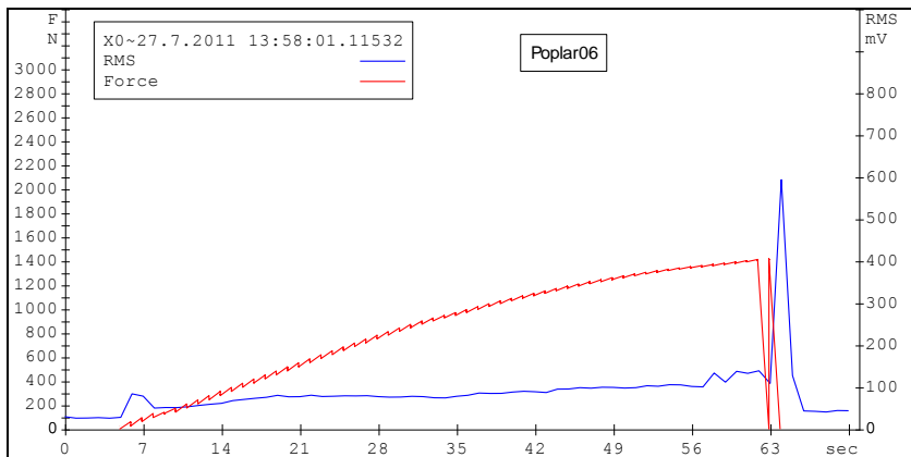
Figure 2: Typical plot of loading force vs. AE RMS for POPLAR specimen group.
